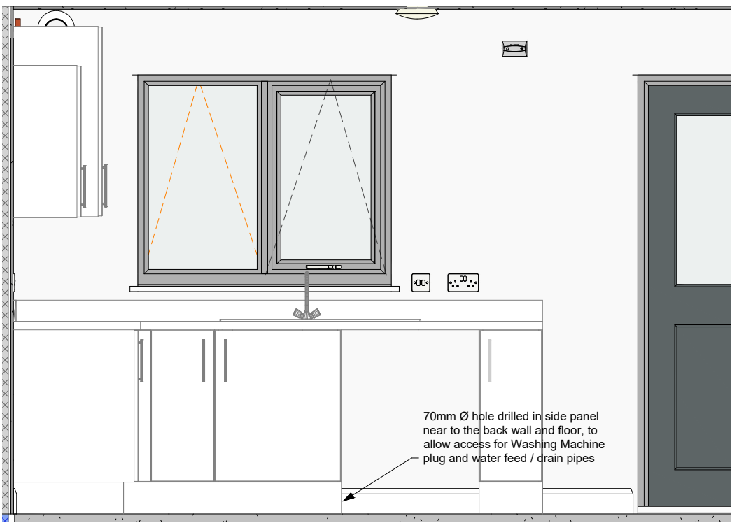
C Kitchen - View C (Rented Spec) 1 : 25
