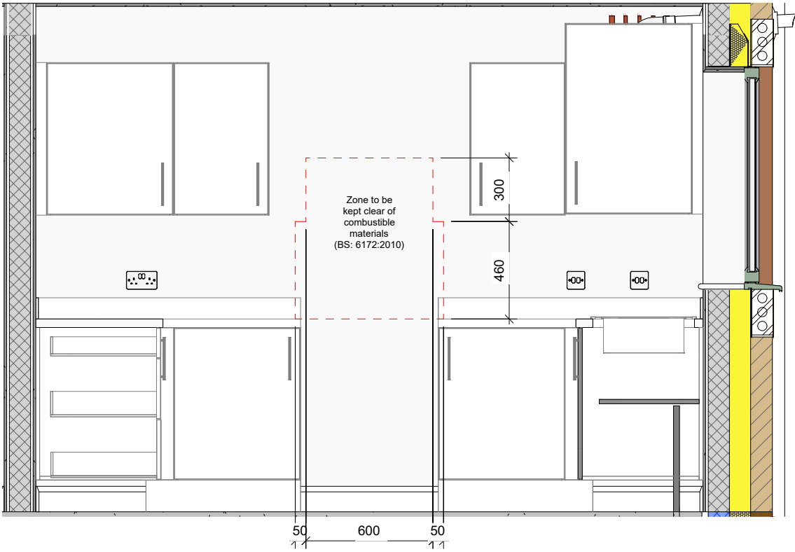
B Kitchen - View B (Rented Spec) 1 : 25
